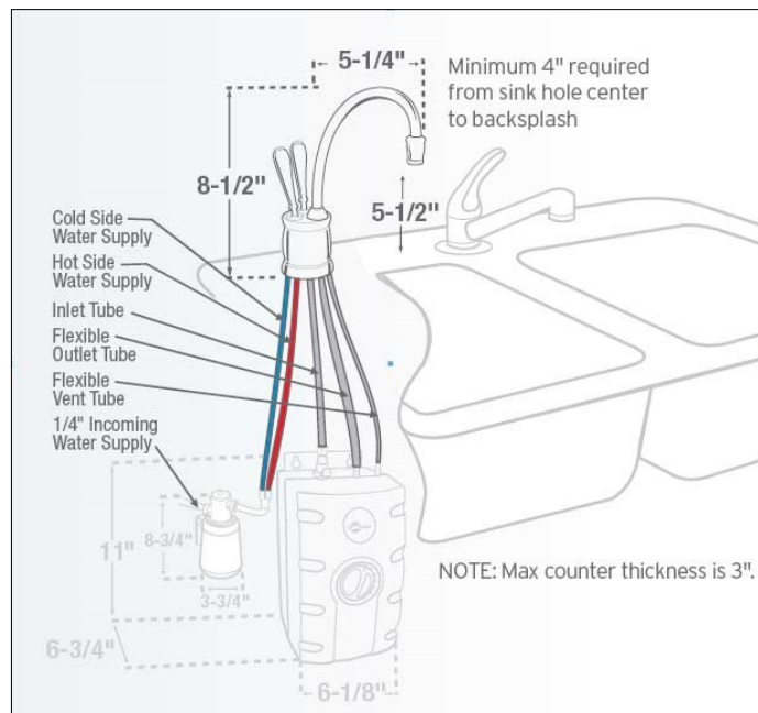
Figure 8-B Hot Tank, Vented Faucet Installation
