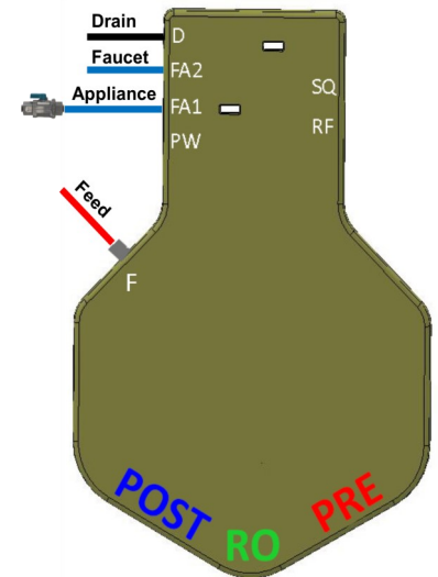
Figure 4: System Connections
