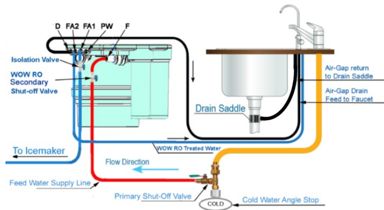
Figure 1: Installation Diagram
